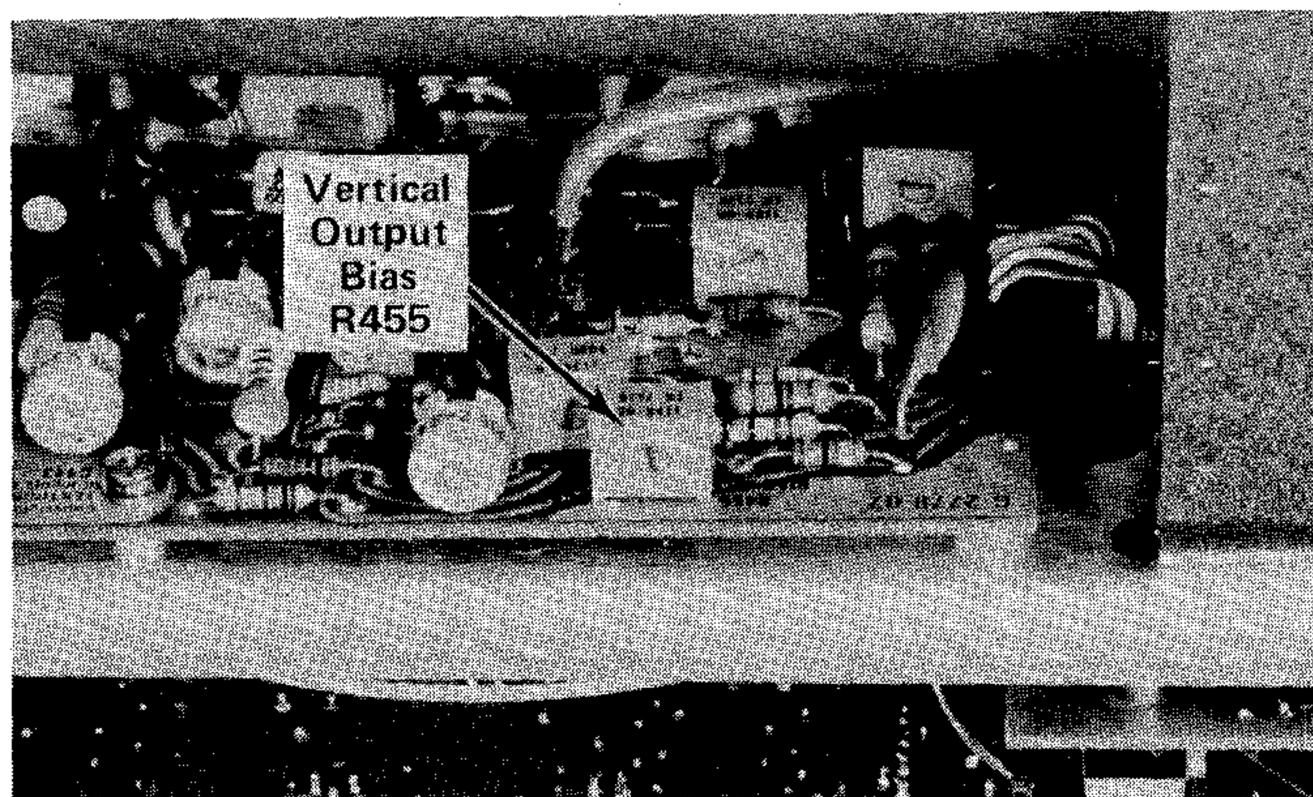
Fig. 5-7. Location of Vertical Output Bias adjustment.
