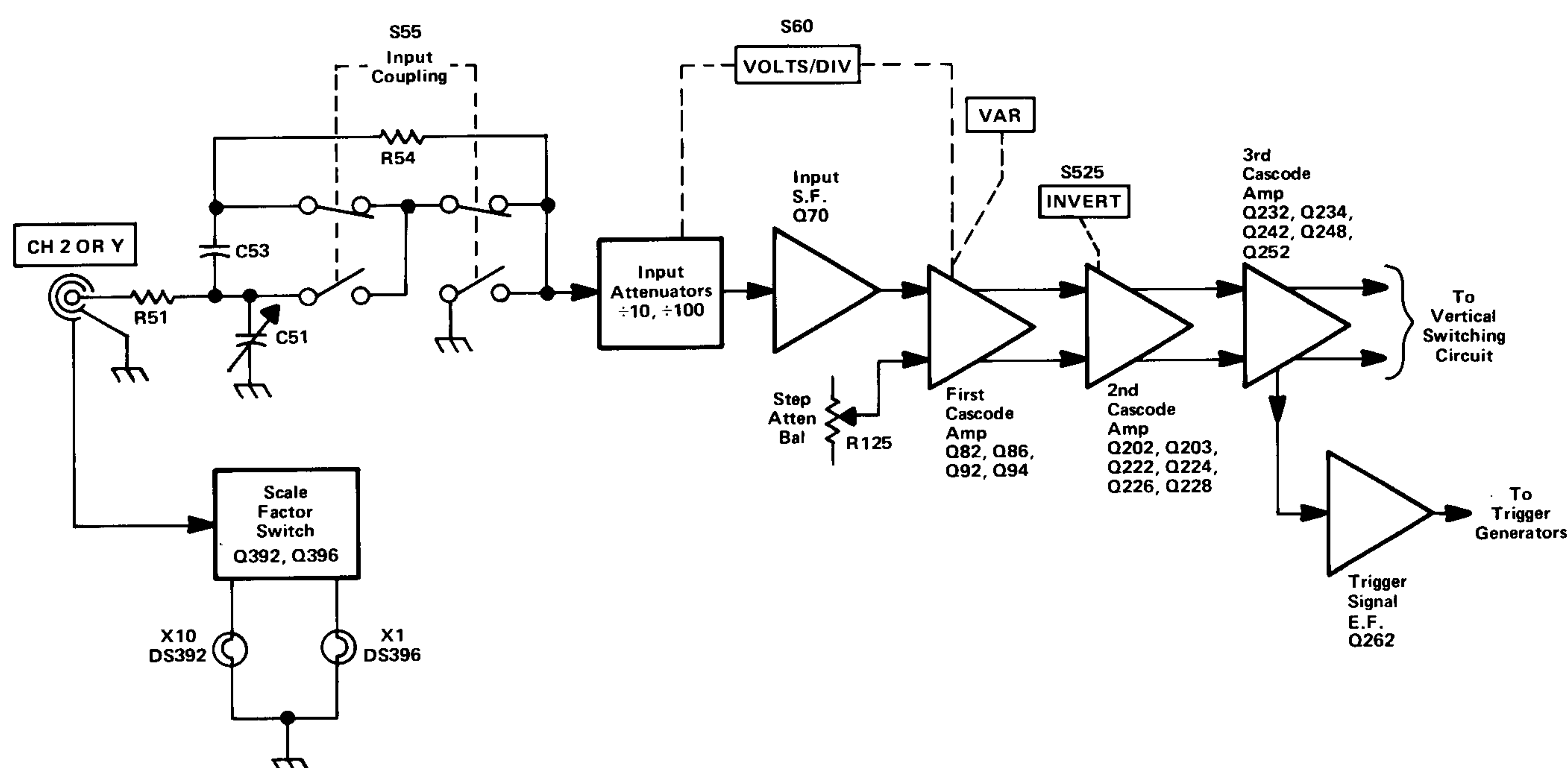
Fig. 3-3. Detailed block diagram of the Channel 2 Preamplifier.
