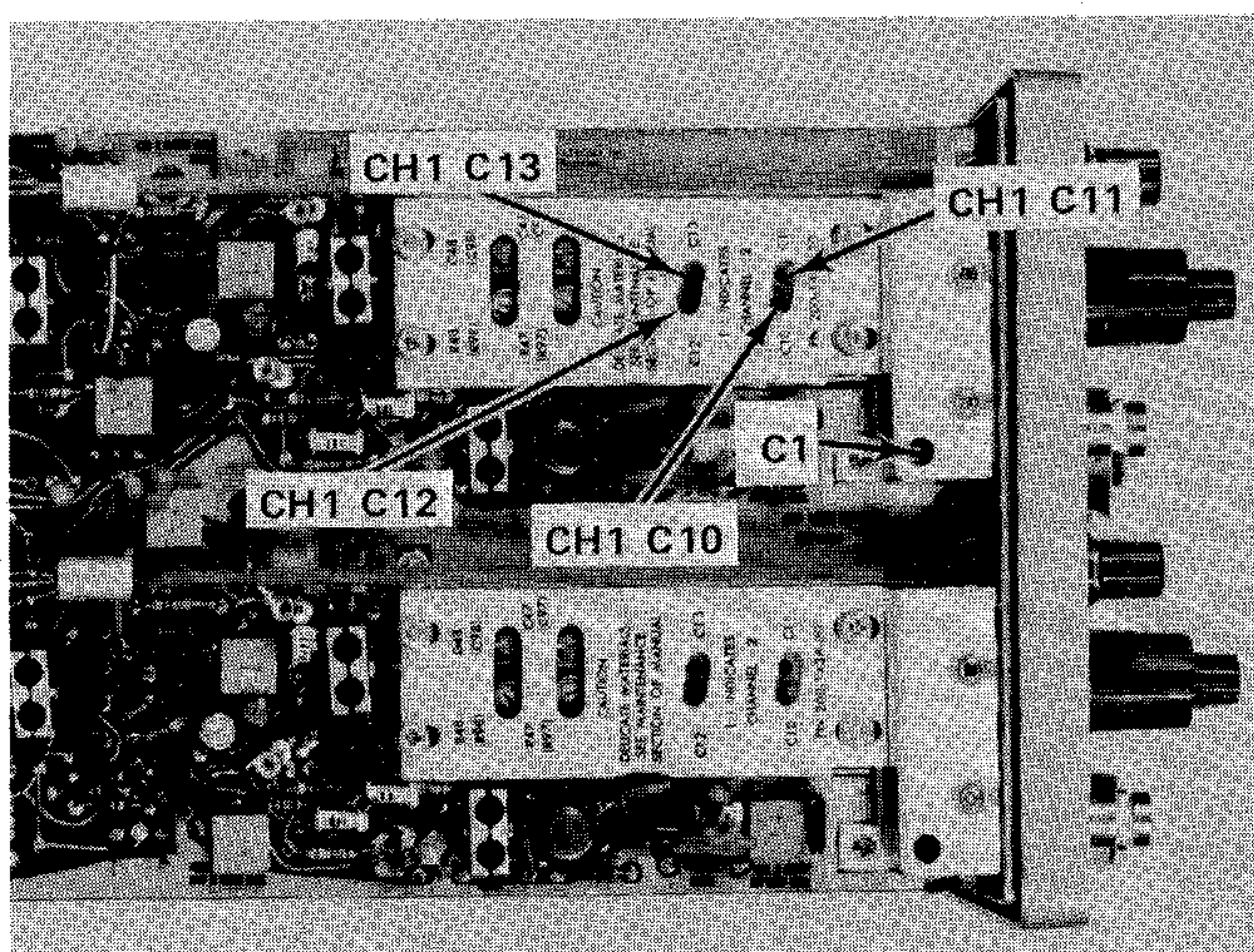
Fig. 5-19. Location of CH 1 volts/div compensation adjustments.
