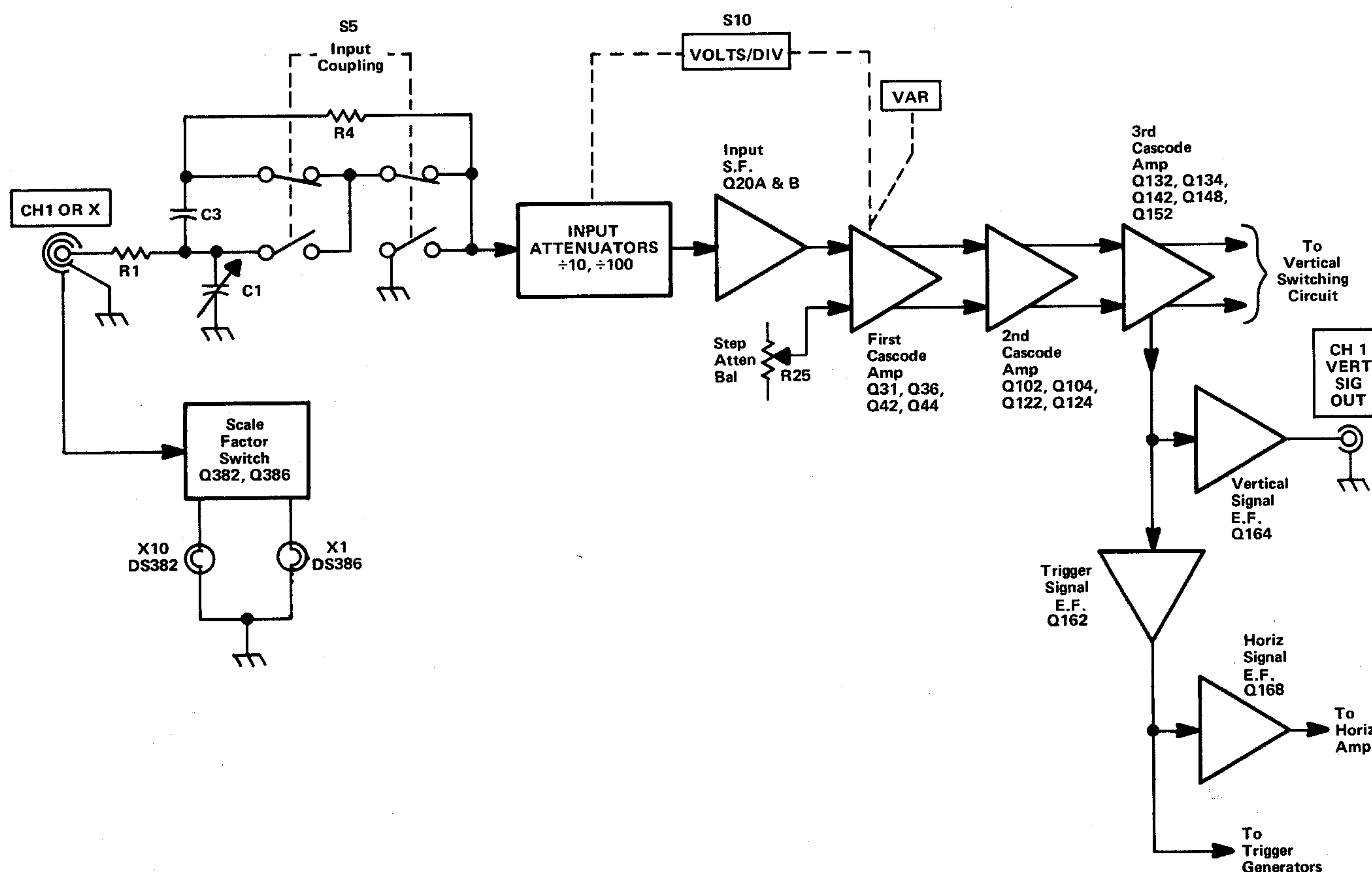
Fig. 3-2. Detailed block diagram of the Channel 1 Preamplifier.
