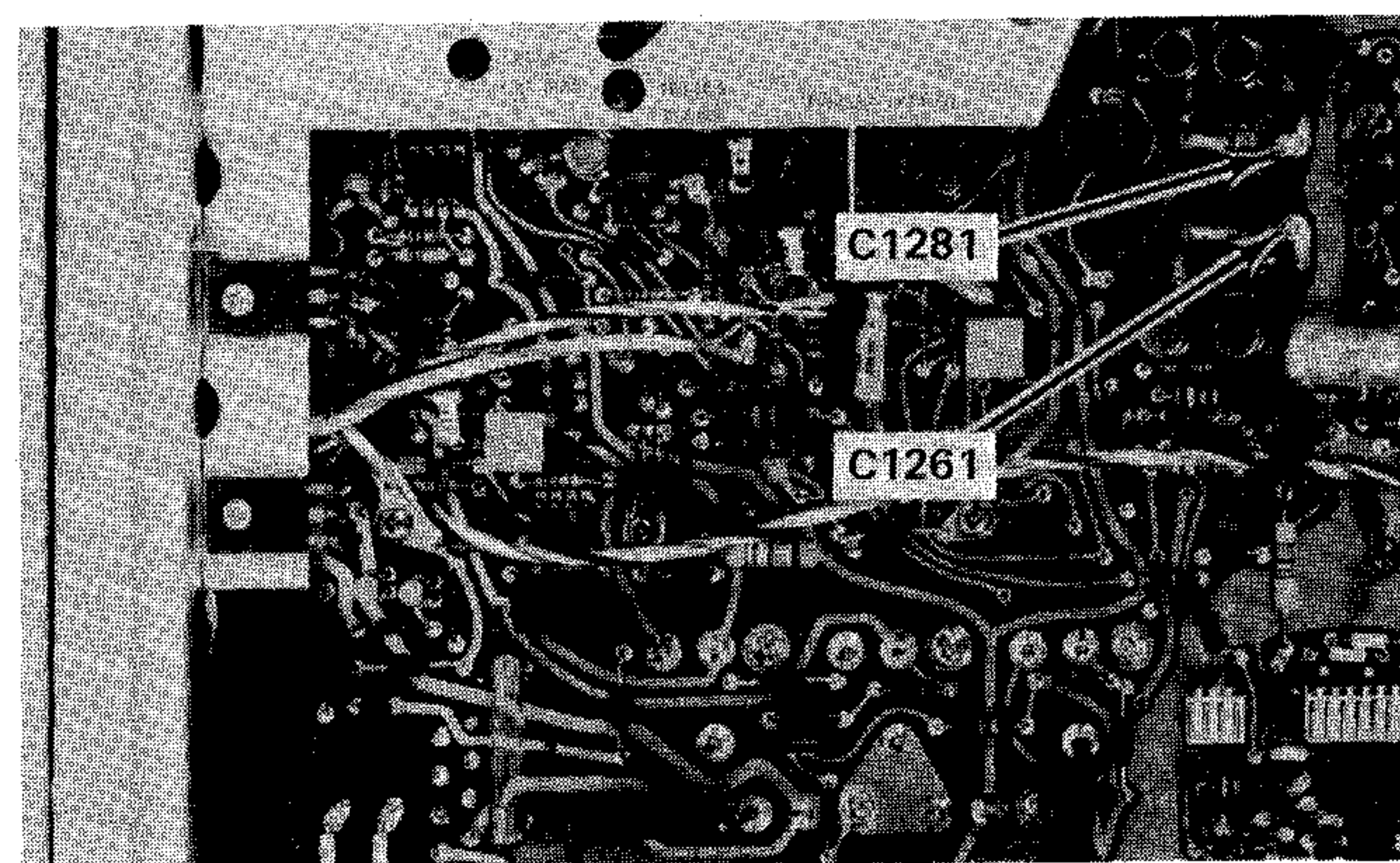
Fig. 5-32. Location of Magnified Timing adjustment.
