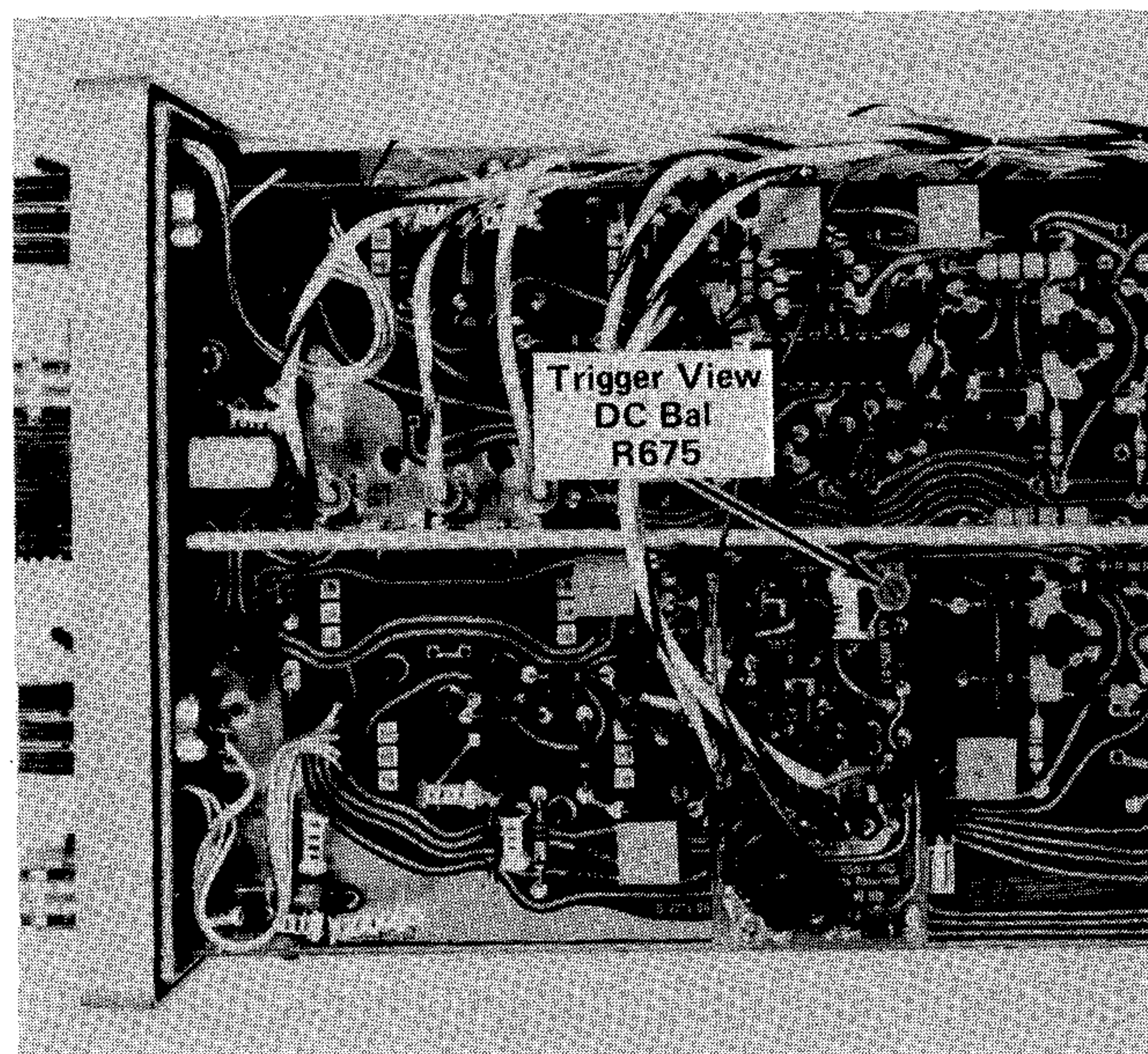
Fig. 5-28. Location of Trigger View Centering adjustment.
