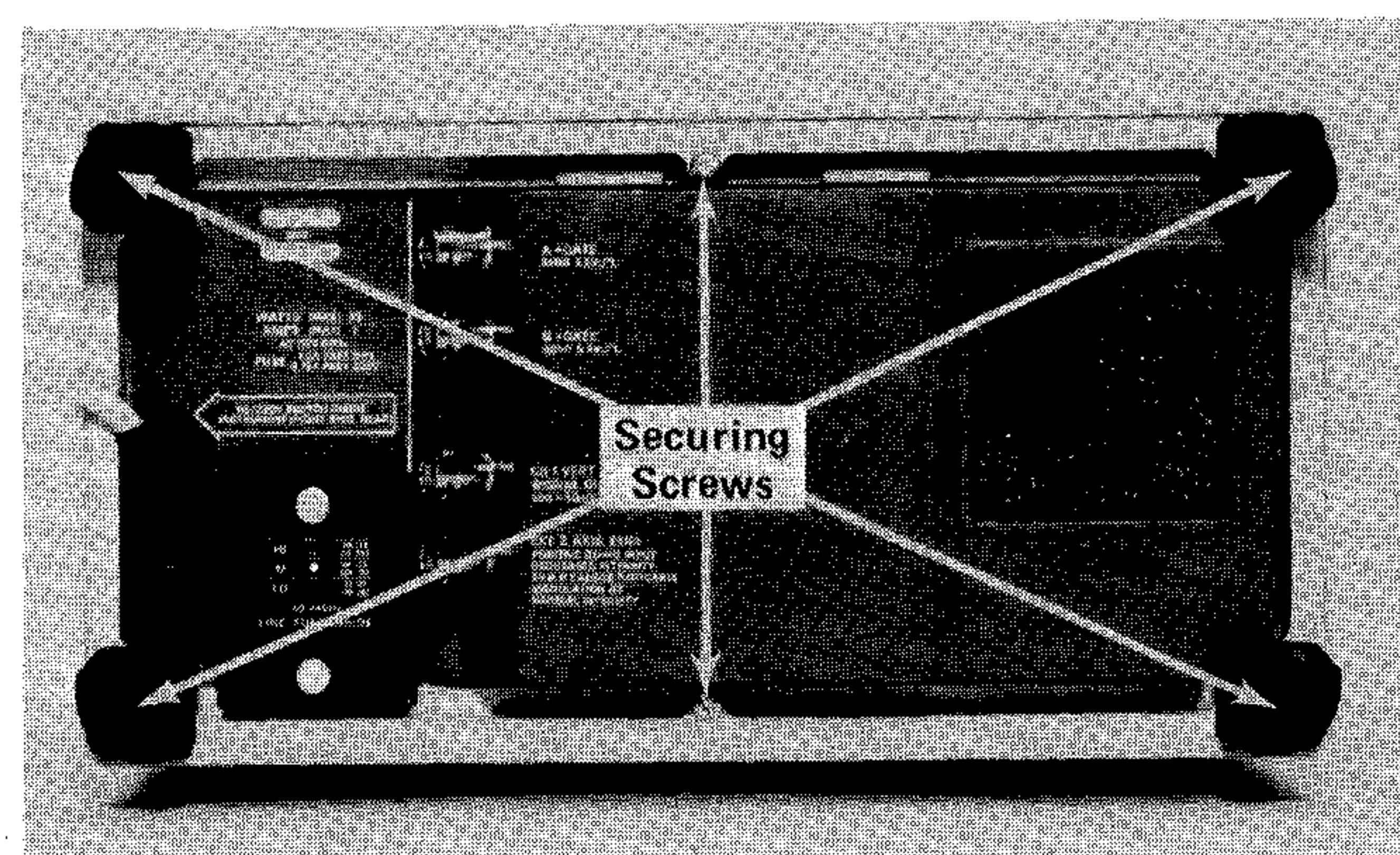
Fig. 4-1. Removing wrap-around cabinet.
