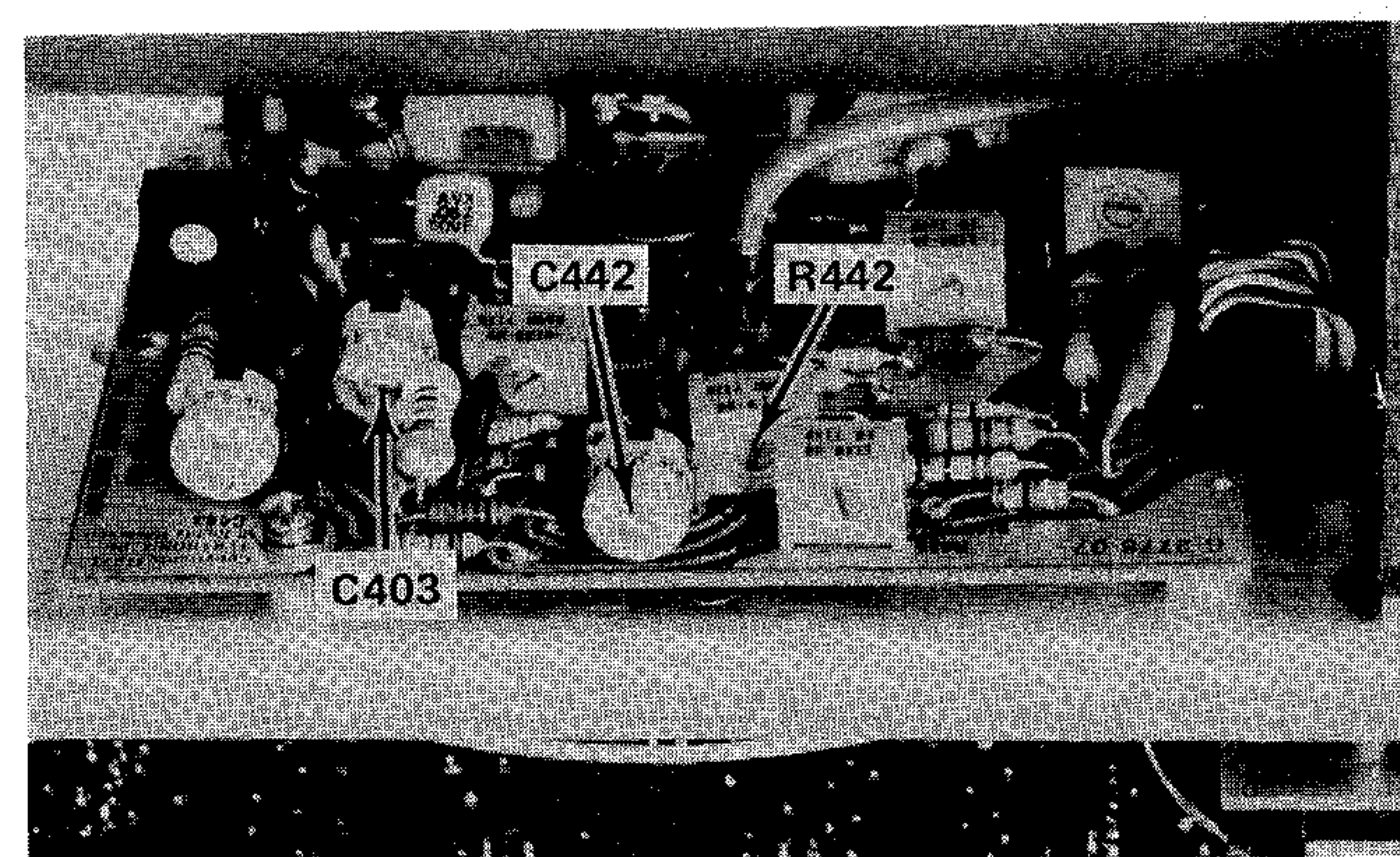
Fig. 5-22. Location of Vertical Output High-Frequency Compensation adjustments.
