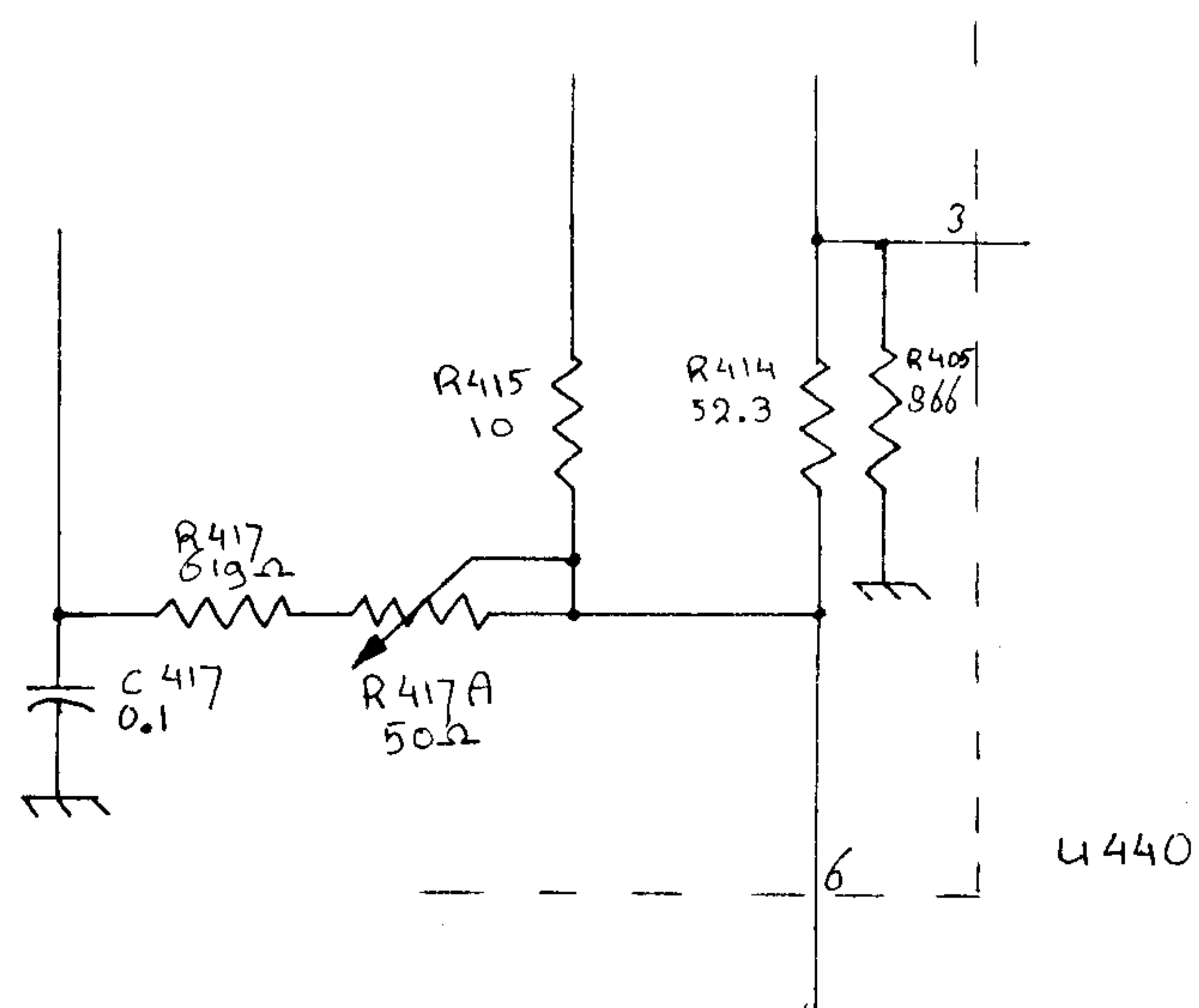
PARTIAL VERTICAL OUTPUT AMPLIFIER
