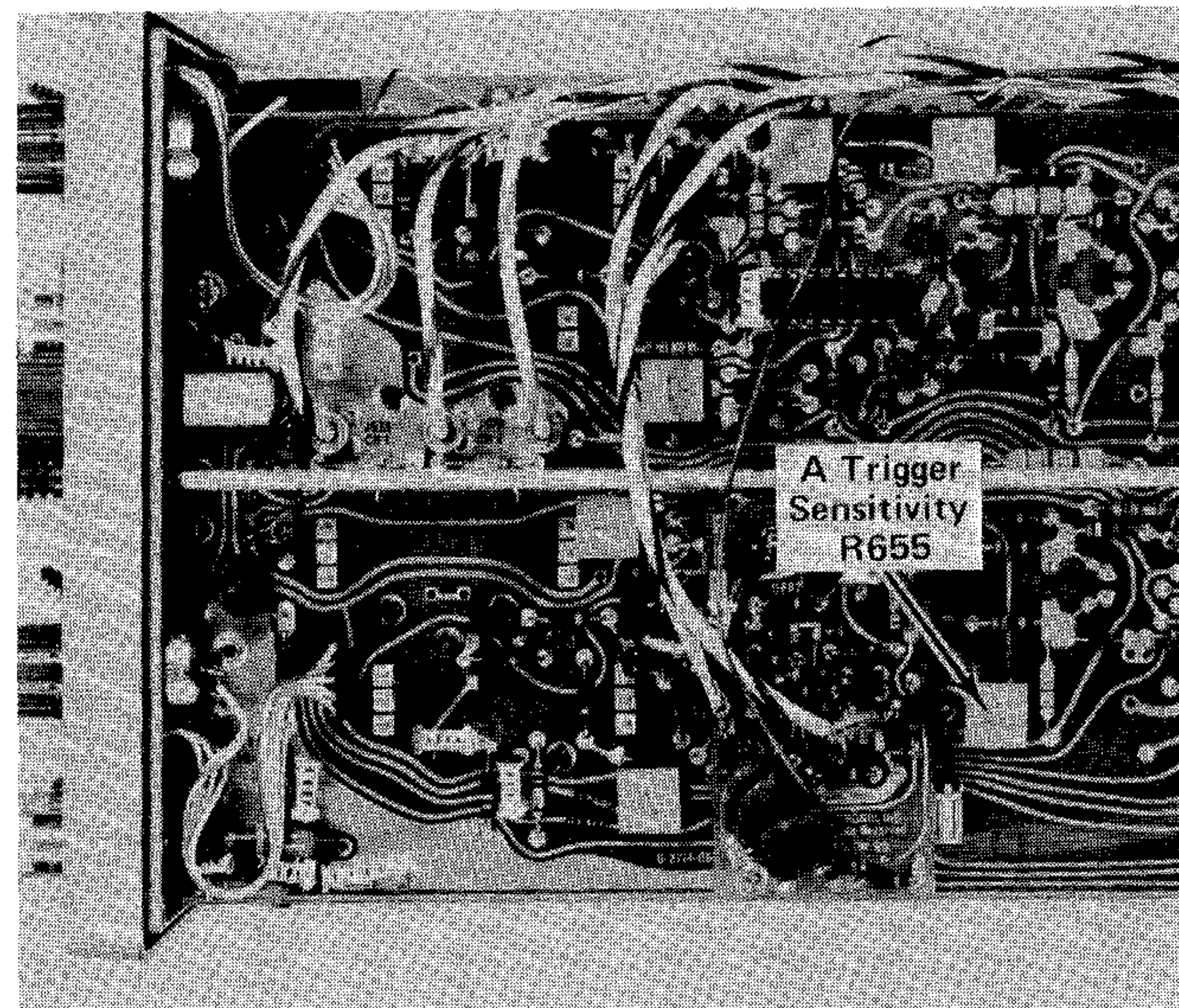
Fig. 5-24. Location of A Trigger Sensitivity adjustment.
