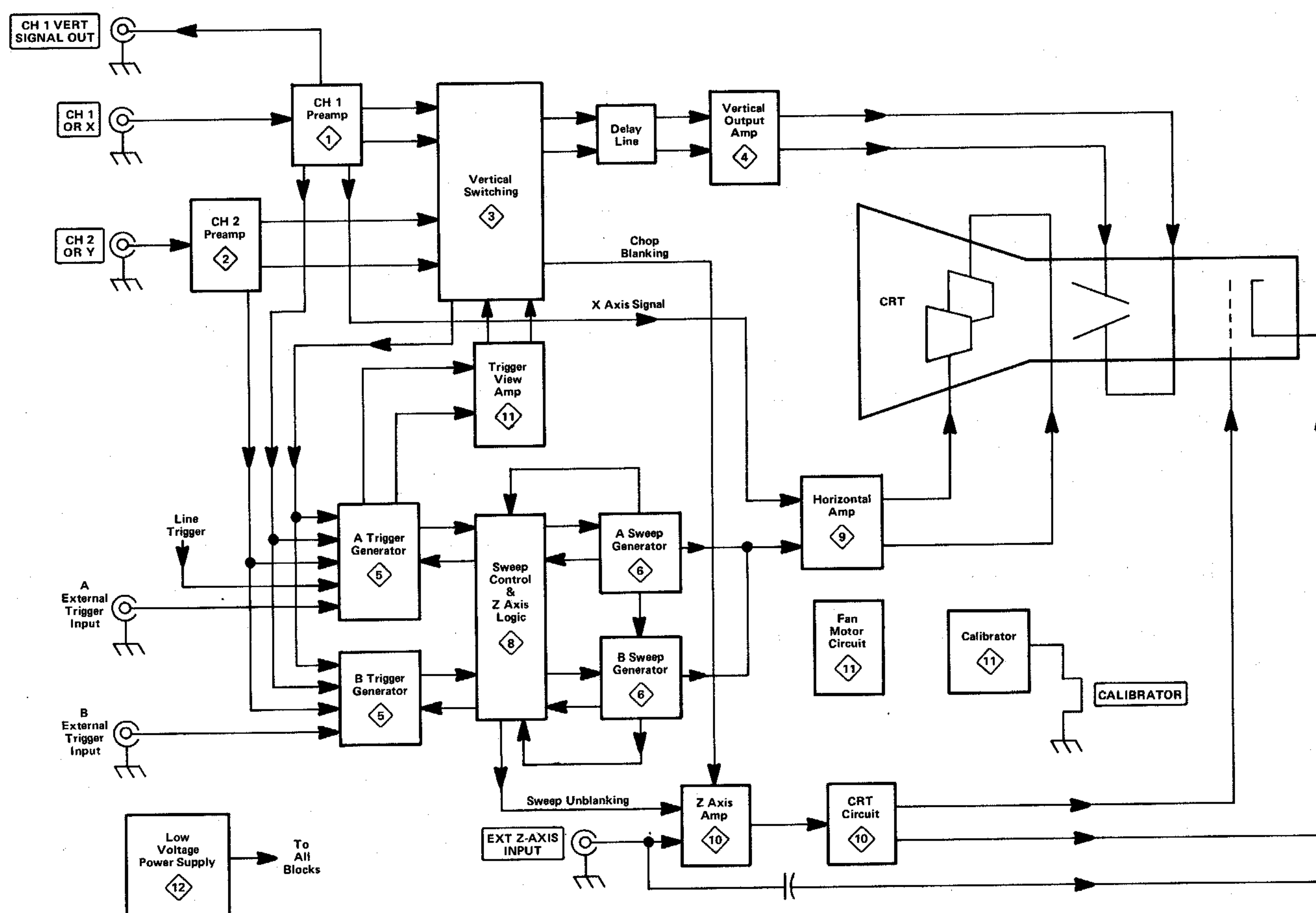
Fig. 3-1. Basic block diagram of the 465.
