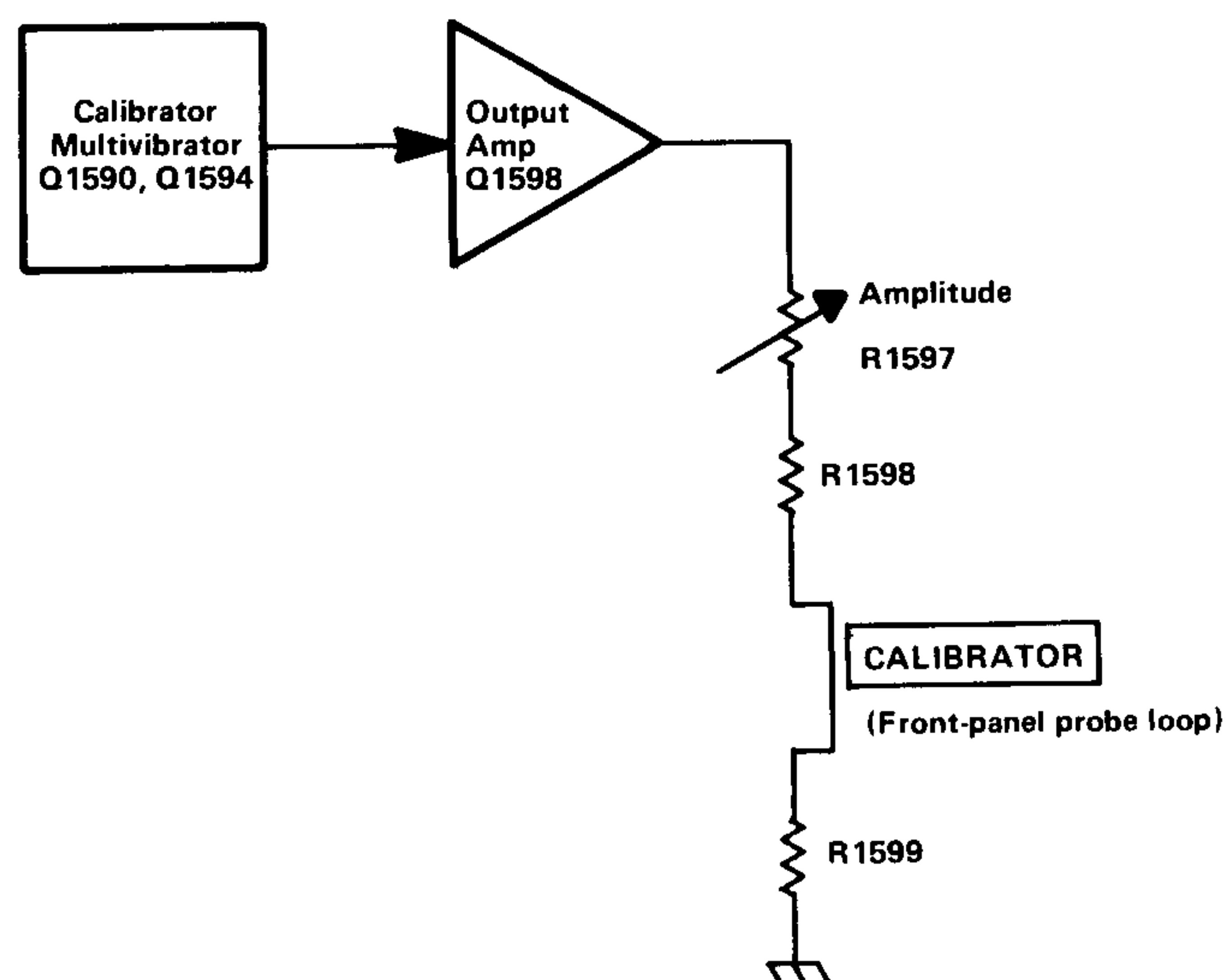
Fig. 3-9. Detailed block diagram of the Calibrator circuit.
