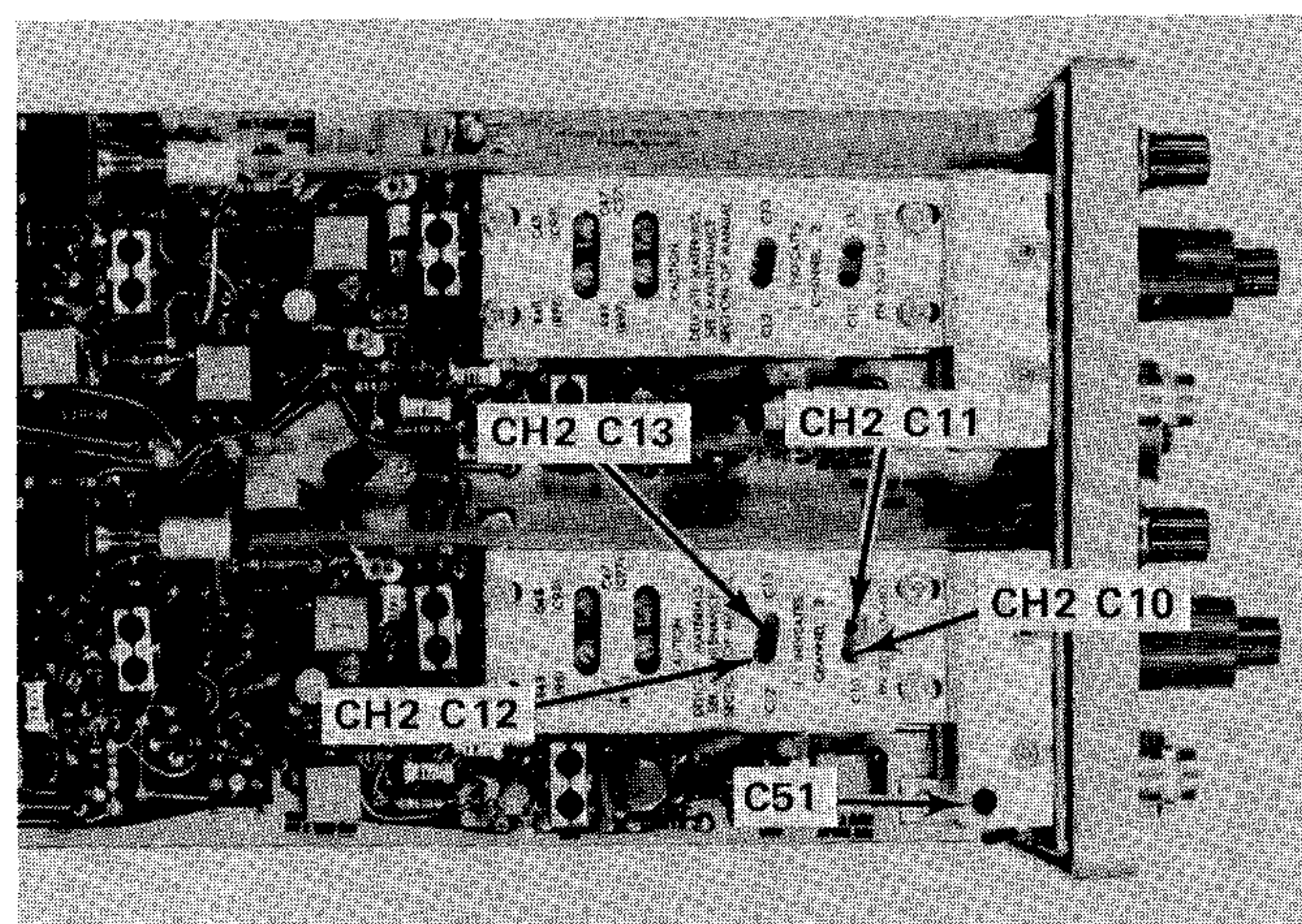
Fig. 5-20. Location of CH 2 volts/div compensation adjustments.
