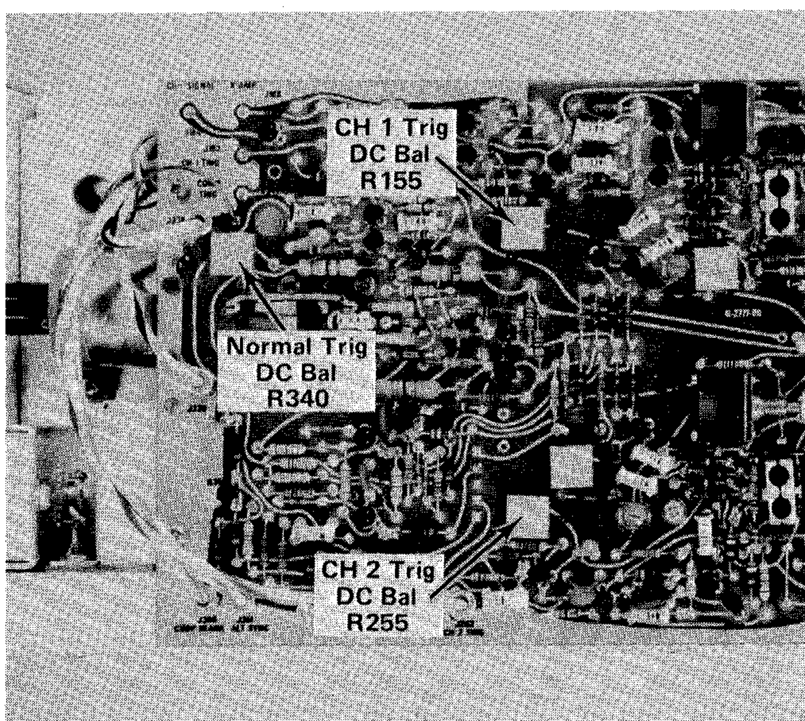
Fig. 5-27. Location of Trigger DC Level adjustments.
