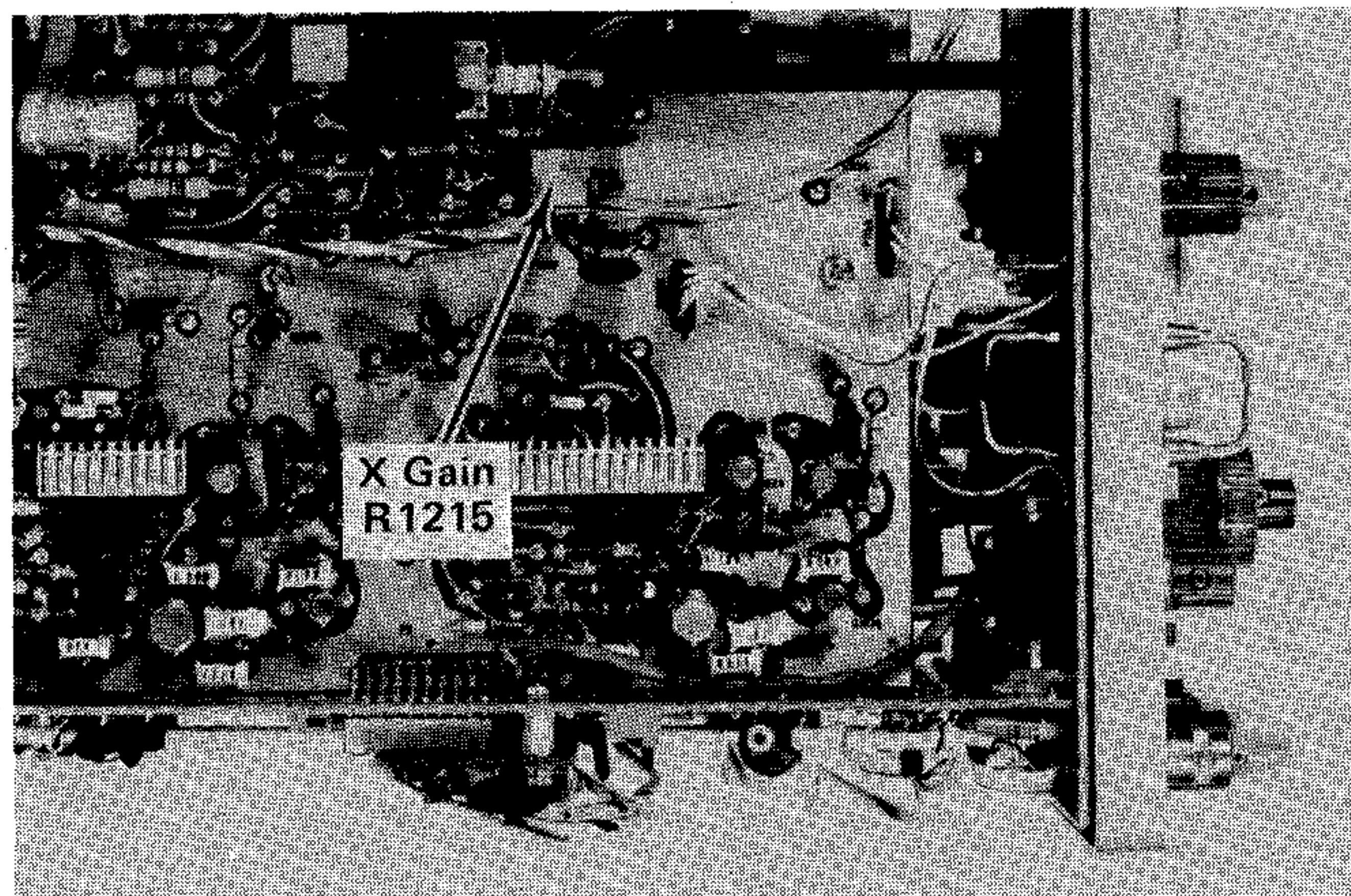
Fig. 5-33. Location of X-Gain adjustment.
