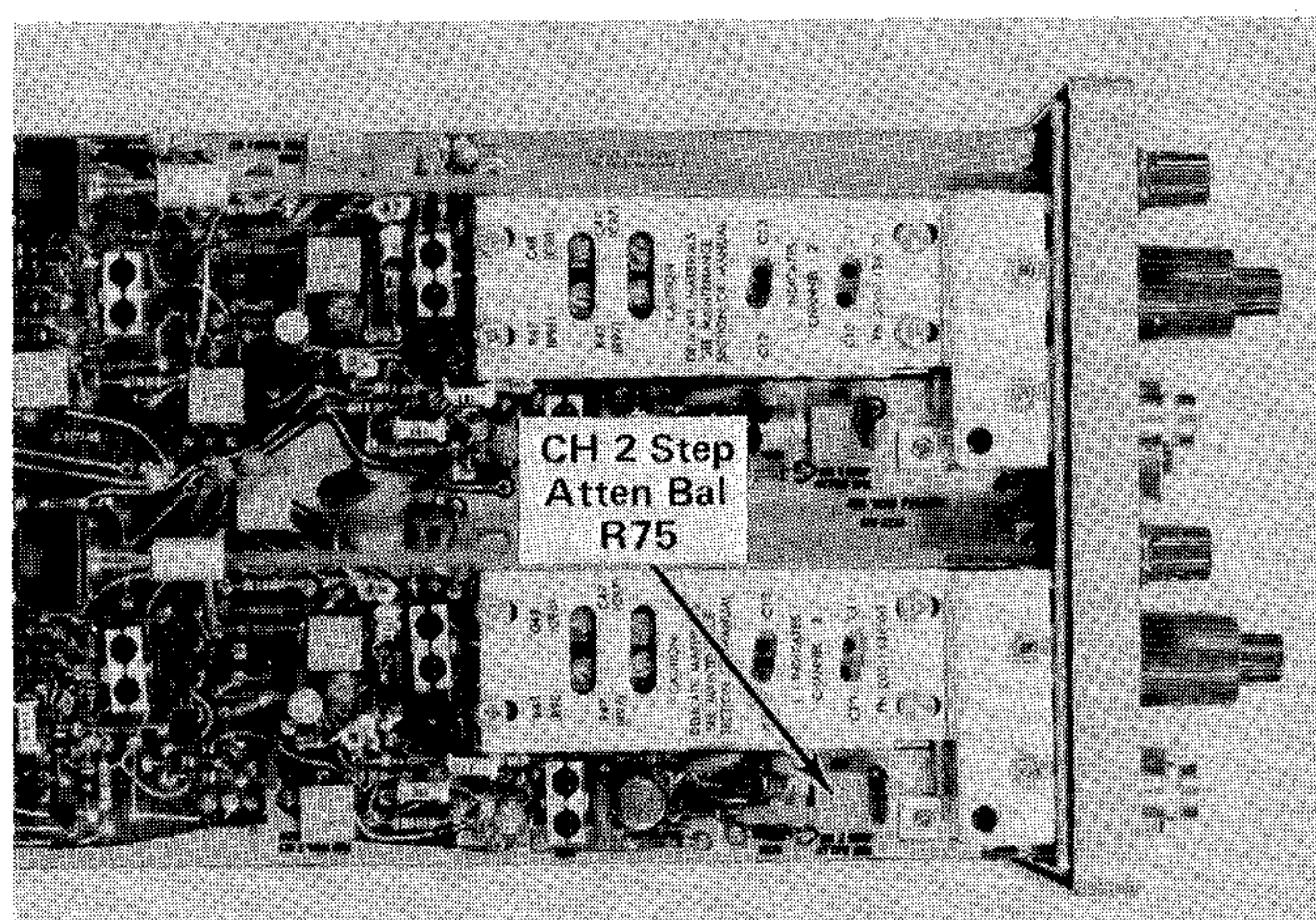
Fig. 5-12. Location of CH 2 Step Atten Bal adjustment.
