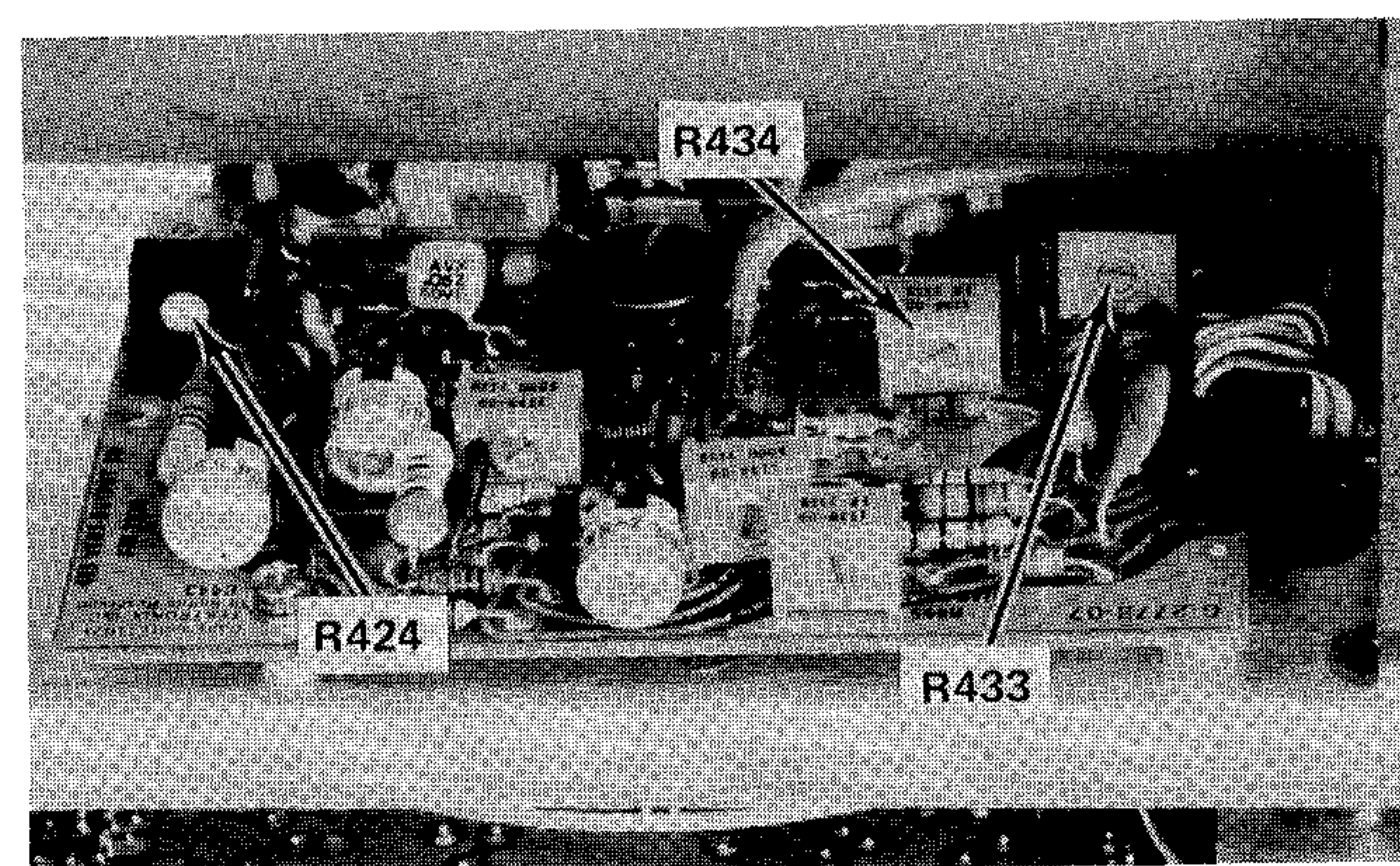
Fig. 5-18. Location of Vertical Output Low-Frequency Compensation adjustments.
