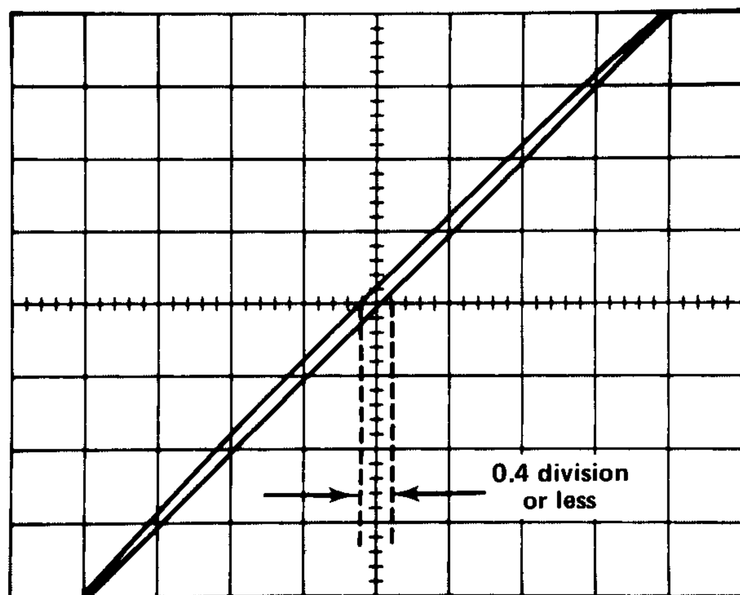
Fig. 5-34. Typical CRT display when checking X-Y phasing.
