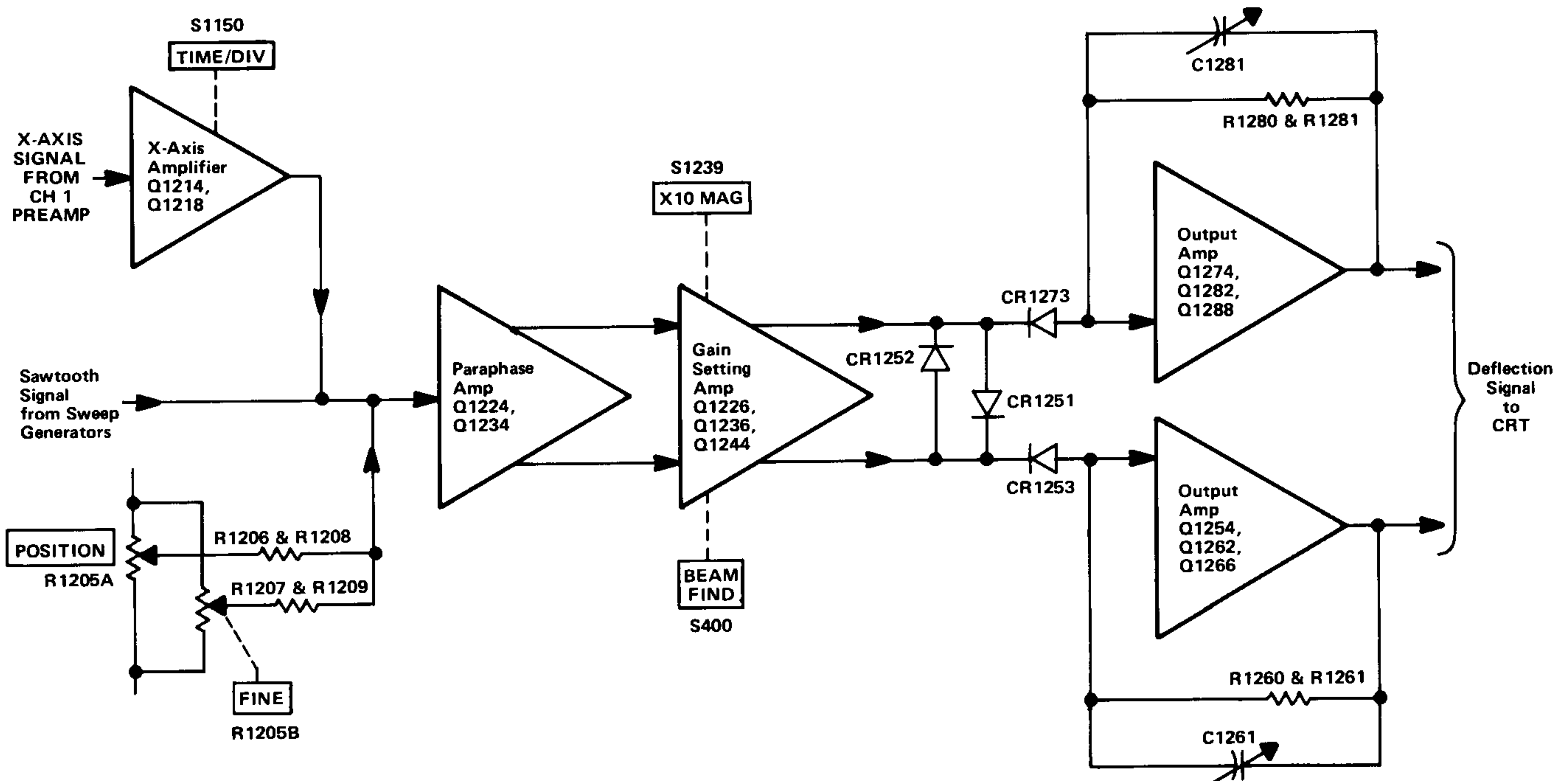
Fig. 3-7. Detailed block diagram of the Horizontal Amplifier.
