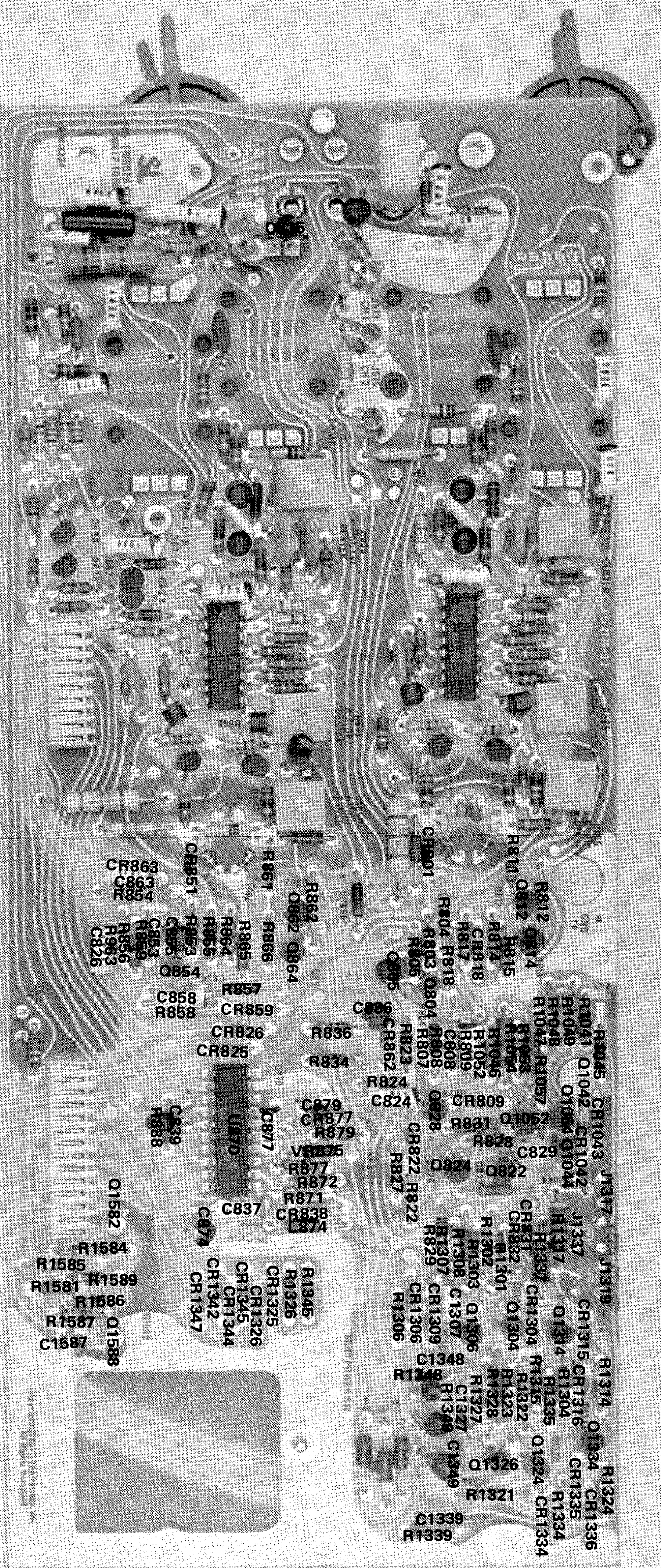
Fig. 7-14A. P/O A8. Trigger Generator & Sweep Logic circuit board, SN B120000-up.
