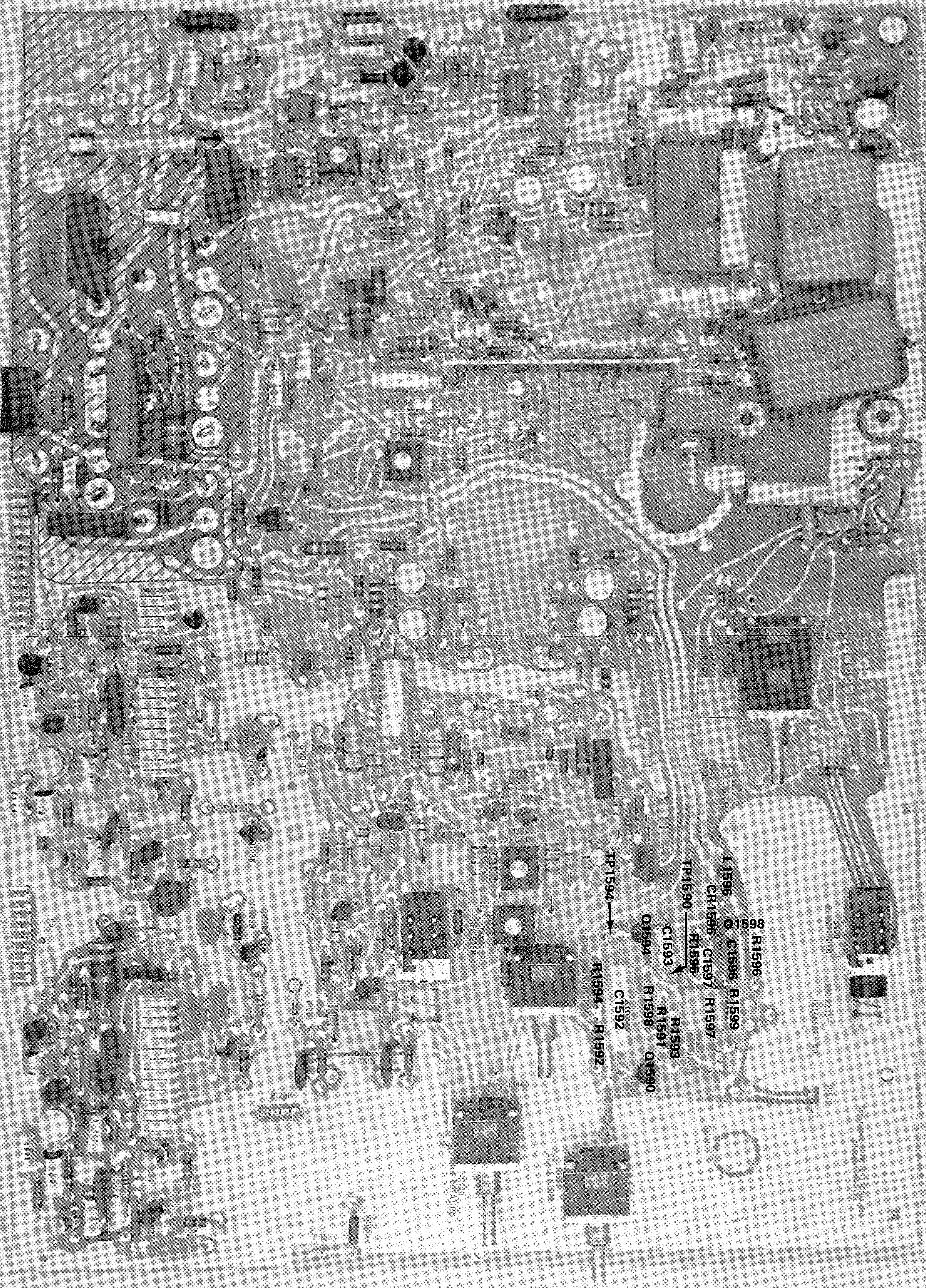
Fig. 7-18A. P/O A9 Interface circuit board SN B080000-up.
