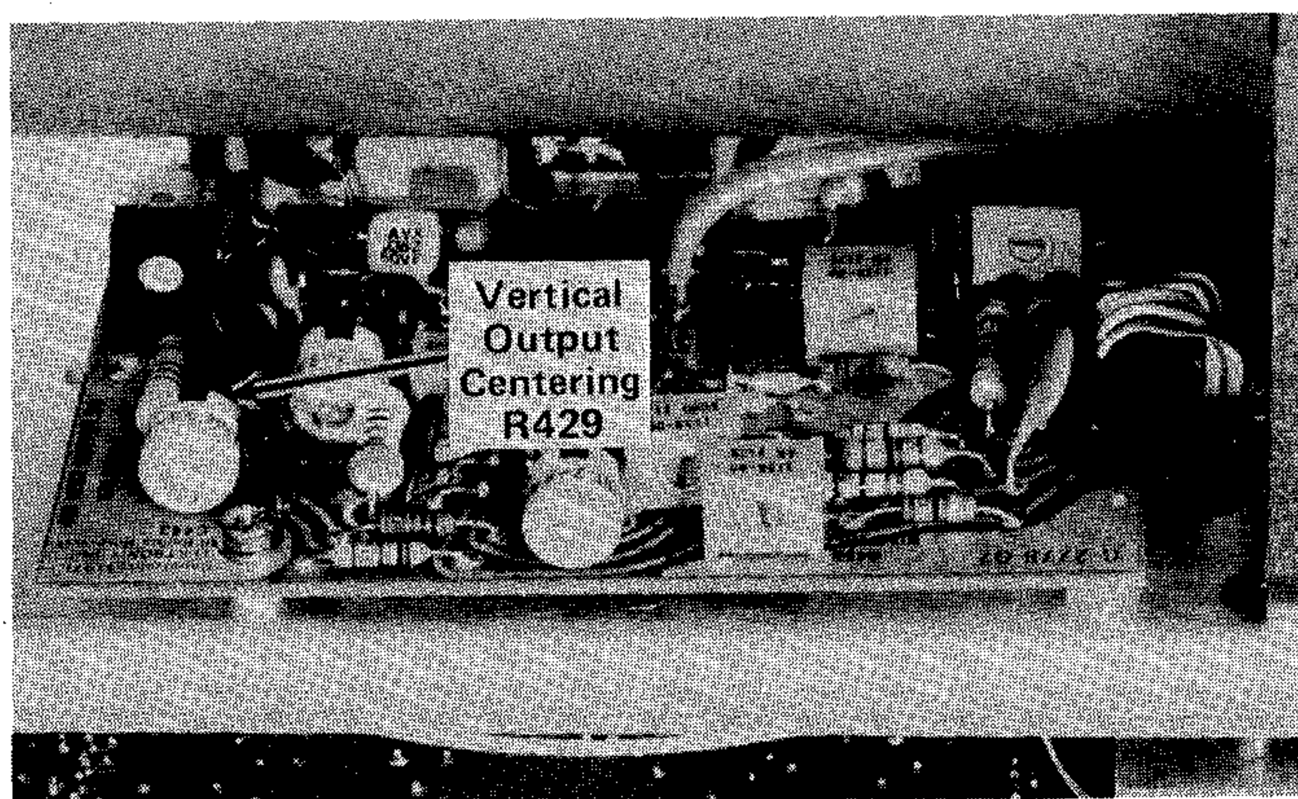
Fig. 5-9. Location of Vertical Output Centering adjustment.
