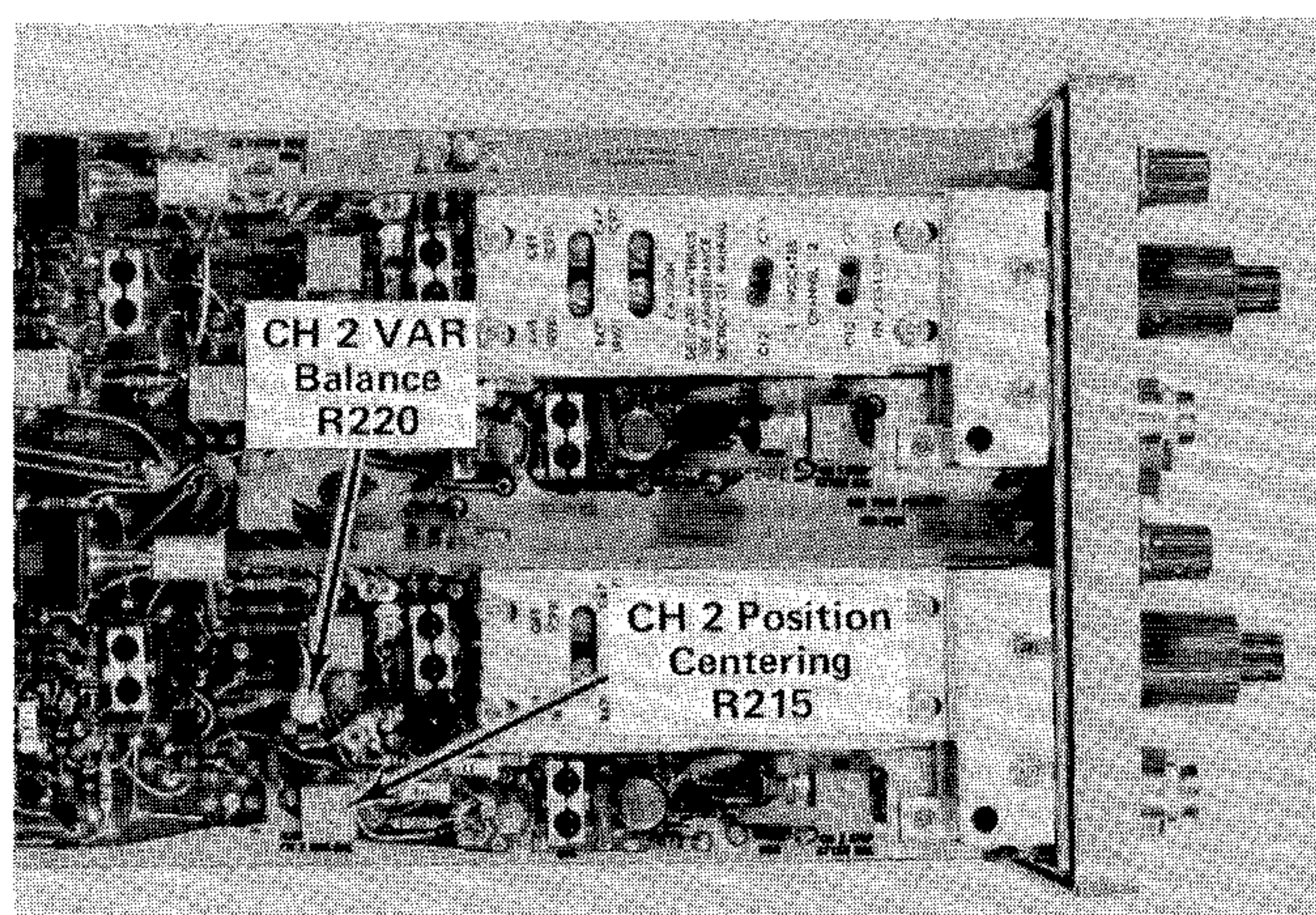
Fig. 5-13. Location of CH 2 Variable Balance and Position Centering adjustments.
