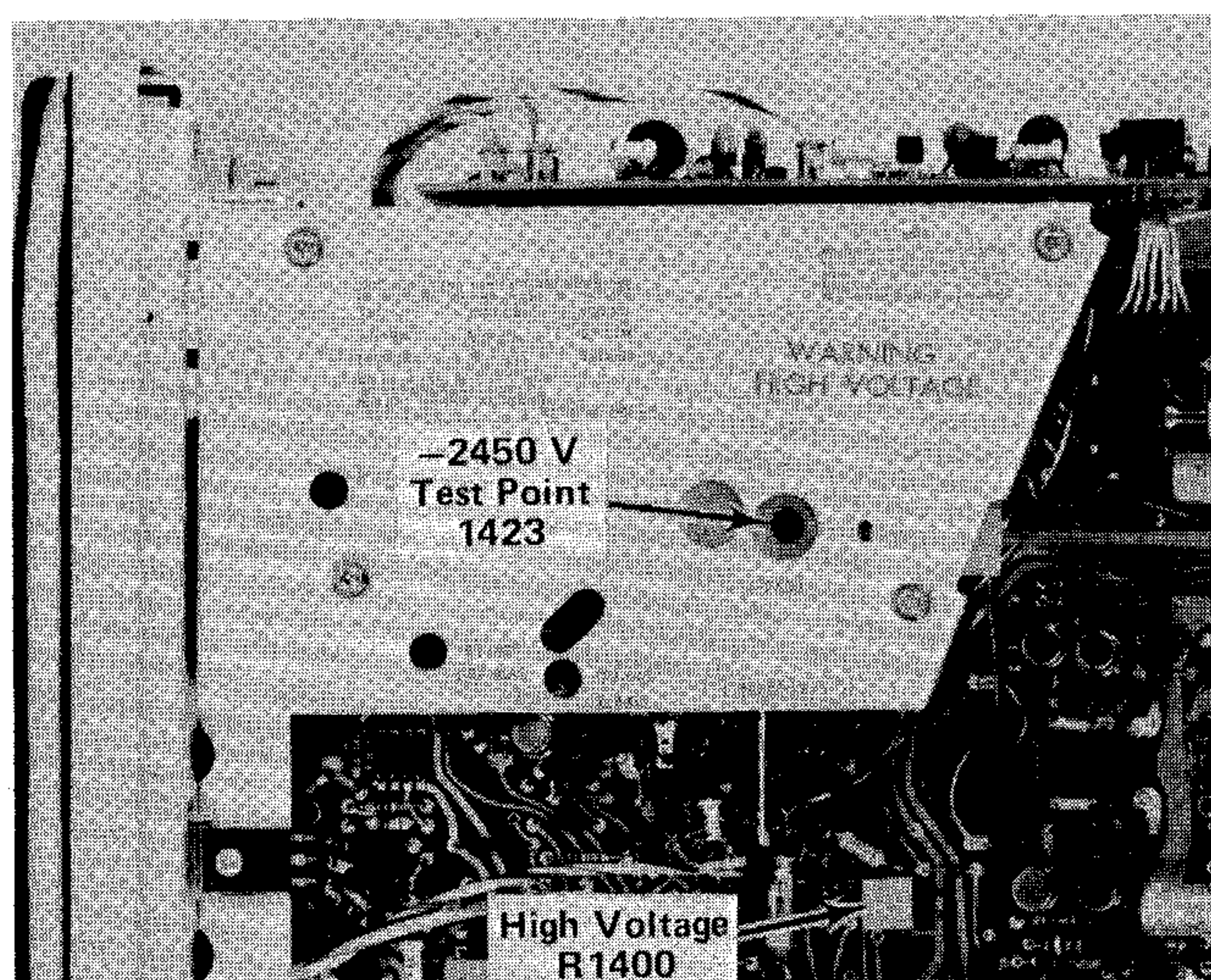
Fig. 5-3. High-voltage test point and adjustment locations.
