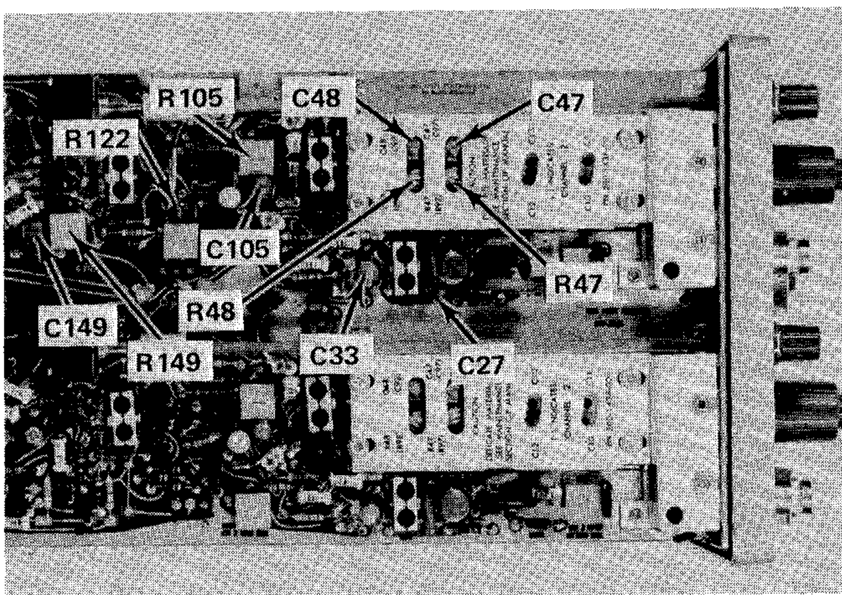
Fig. 5-23. Location of CH 1 High-Frequency Compensation adjustment.
