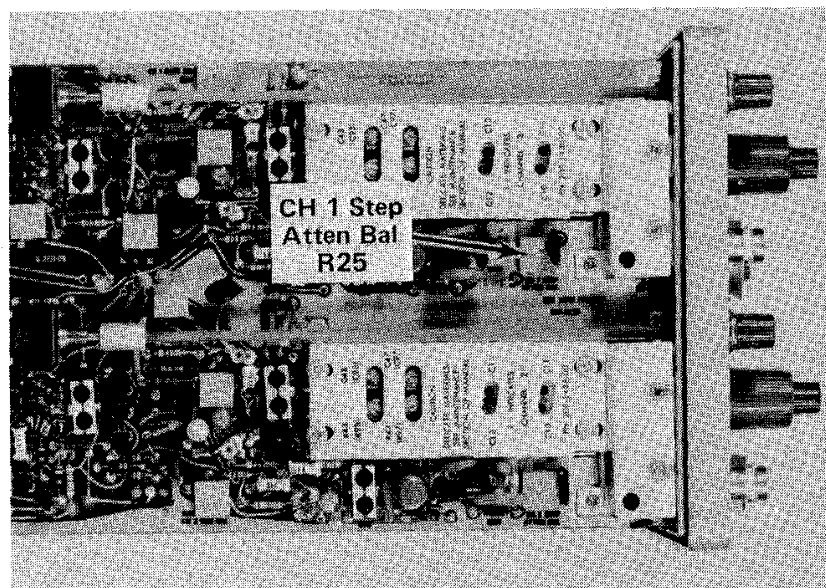
Fig. 5-10. Location of CH 1 Step Atten Bal adjustment.
