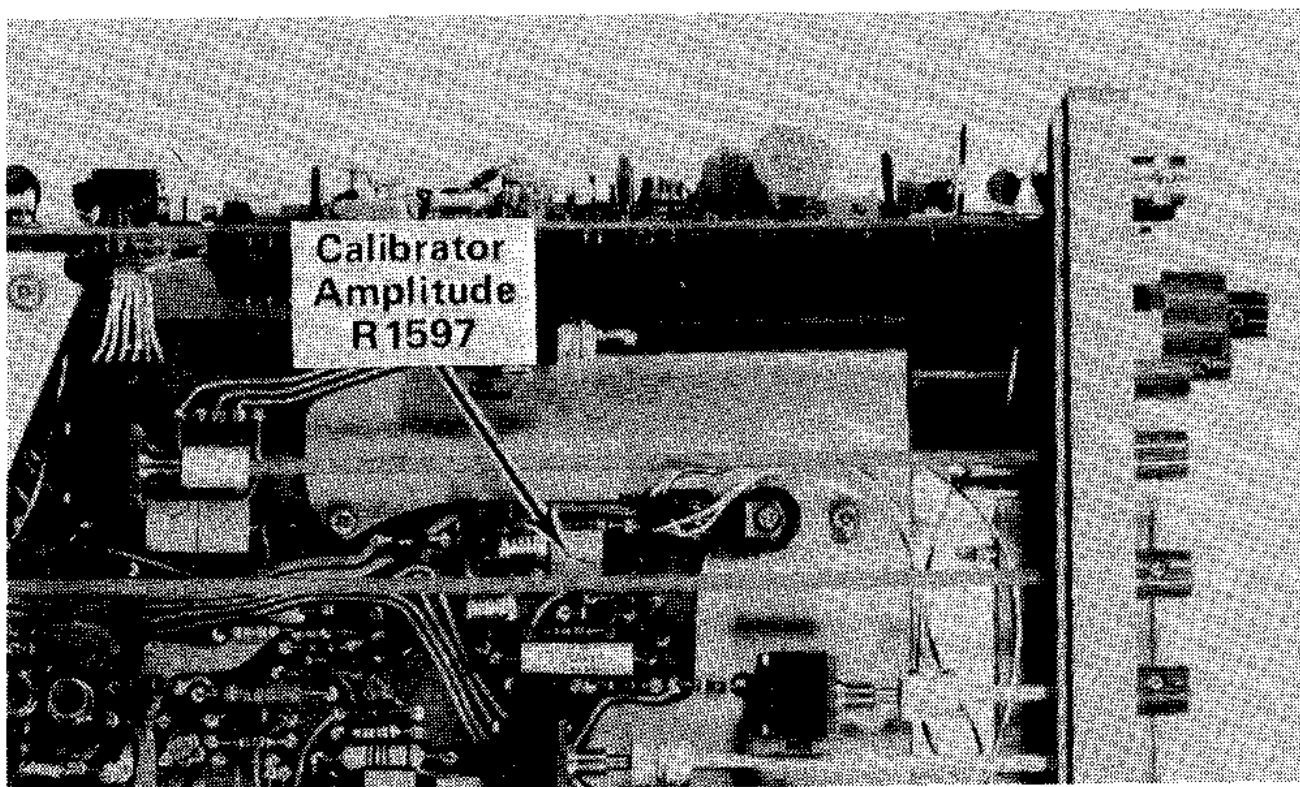
Fig. 5-35. Location of CALIBRATOR Amplitude adjustment.
