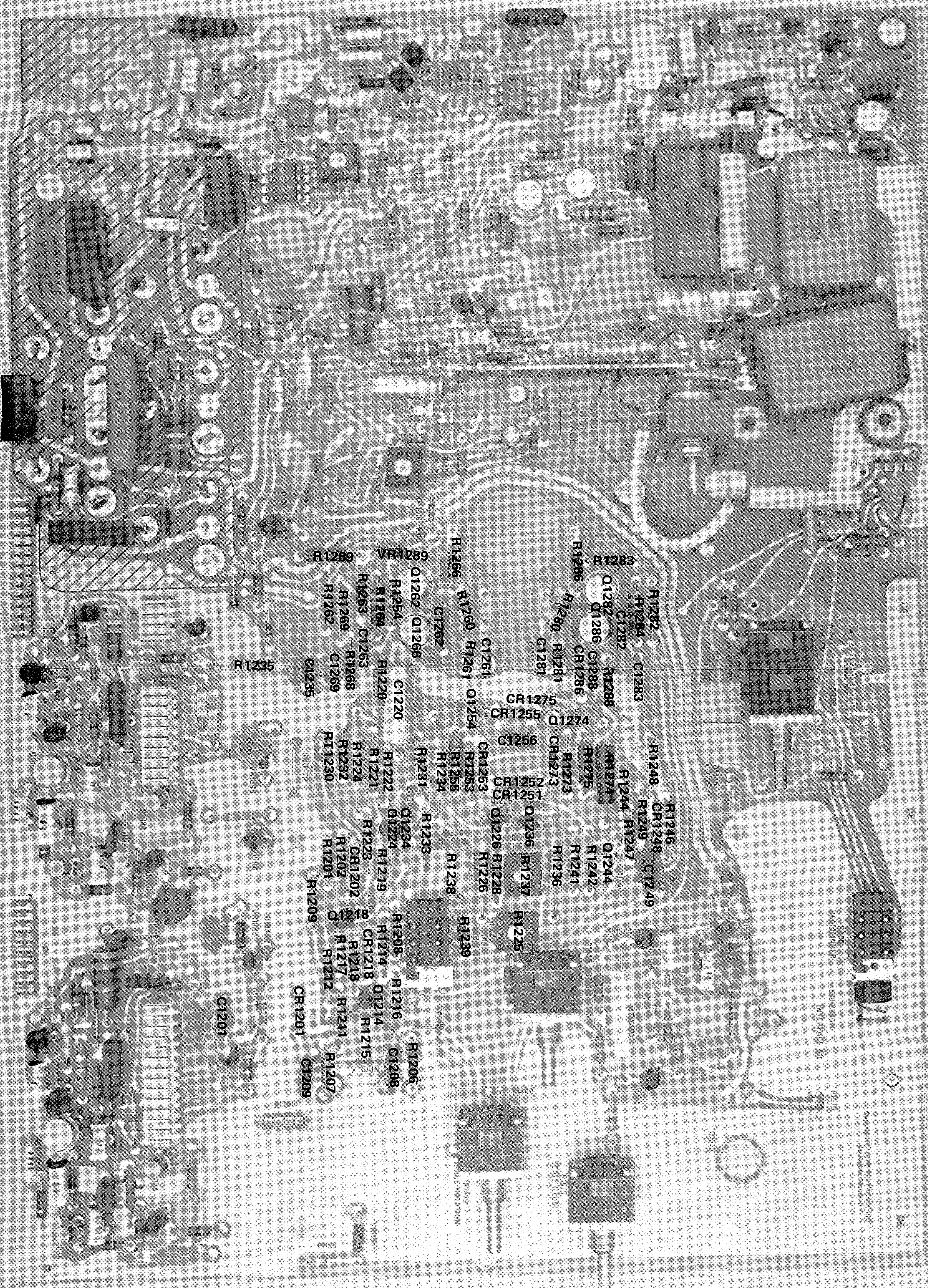
Fig. 7-16A. P/O A9 Interface circuit board SN B080000-up.
